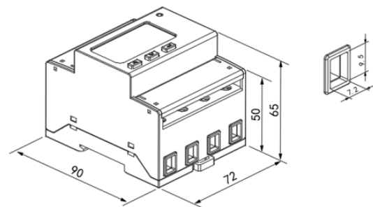
direct connect
